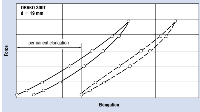
Fig. 40: Rope strength / rope elongation parameters DRAKO 300 T
