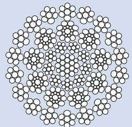
Fig. 14: Rotation-resistant rope constructions (example)
